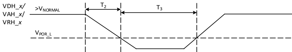
Figure 4-4 Power-off sequence
