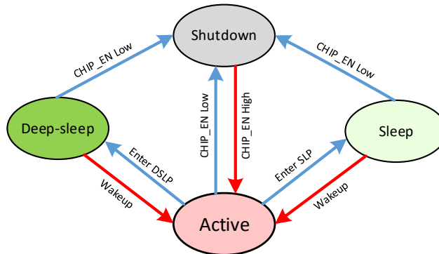
Figure 3-4 Switch among different power modes
