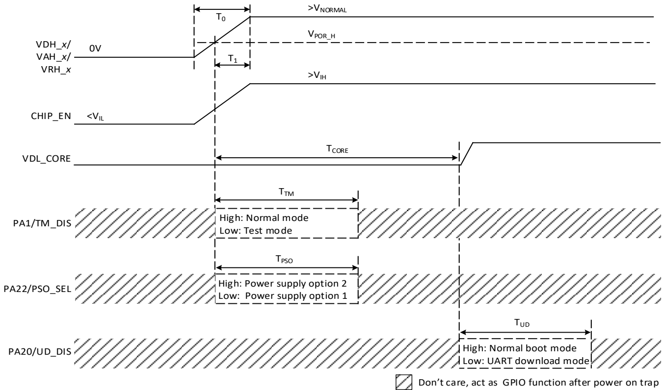
Figure 4-3 Power-on sequence
