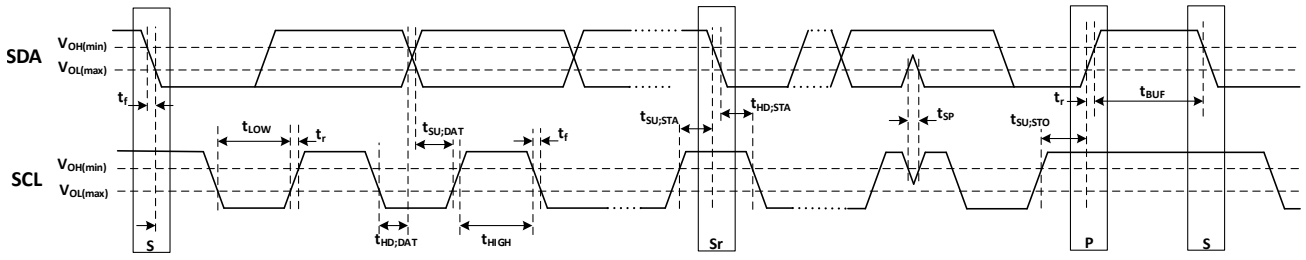
Figure 4-14 Timing diagram of I2C (FS/SS mode)
