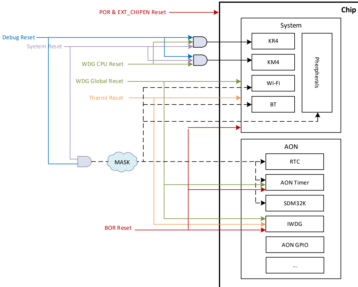
Figure 3-5 Reset diagram
