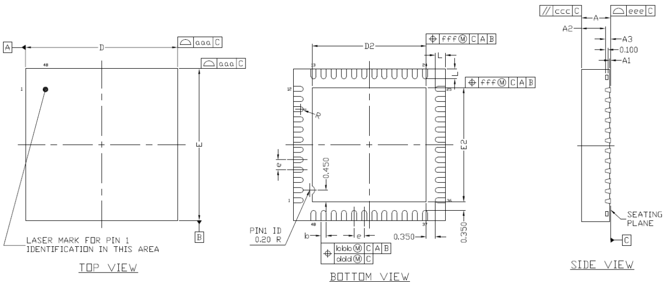
Figure 5-1 QFN48 package outline
