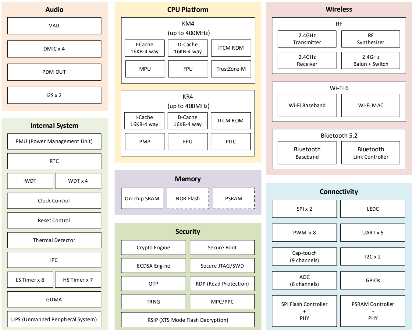
Figure 1-1 Block diagram
