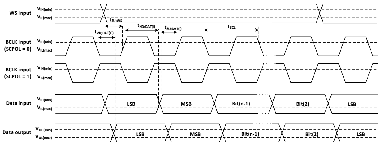
Figure 4-18 Timing diagram for I2S slave
