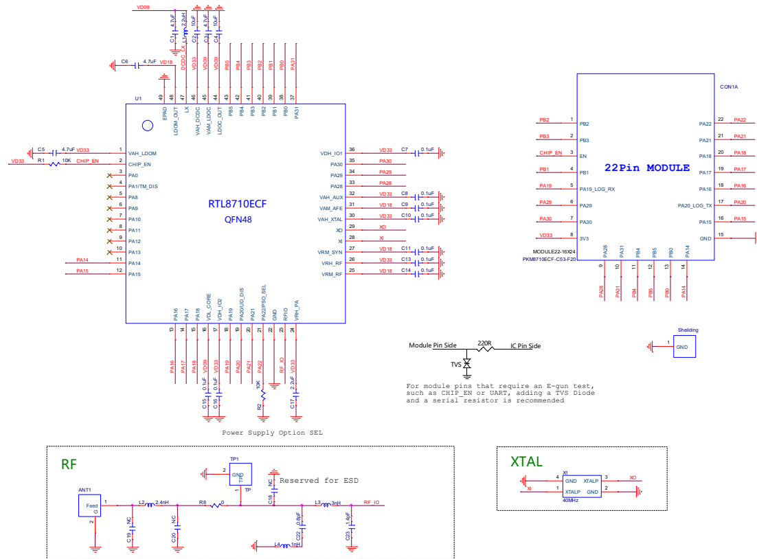
Figure 3.1 PKM8710ECF-C53-F20 Module internal schematics
