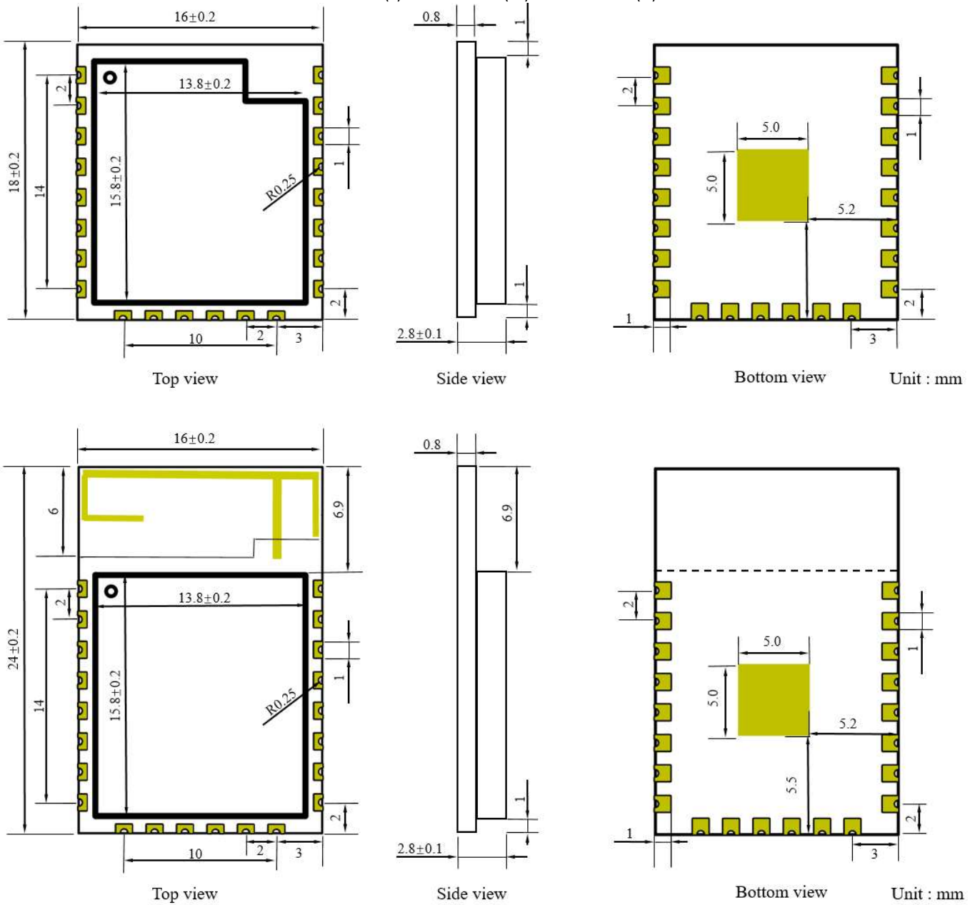
Figure 6. Module Physical Dimensions
