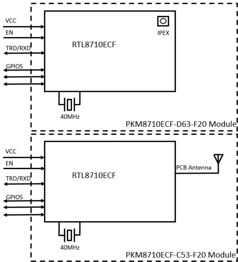
Figure 1. Block Diagram
