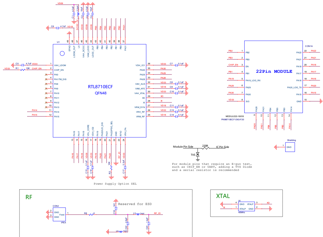
Figure 4.2 PKM8710ECF-D63-F20 Module internal schematics
