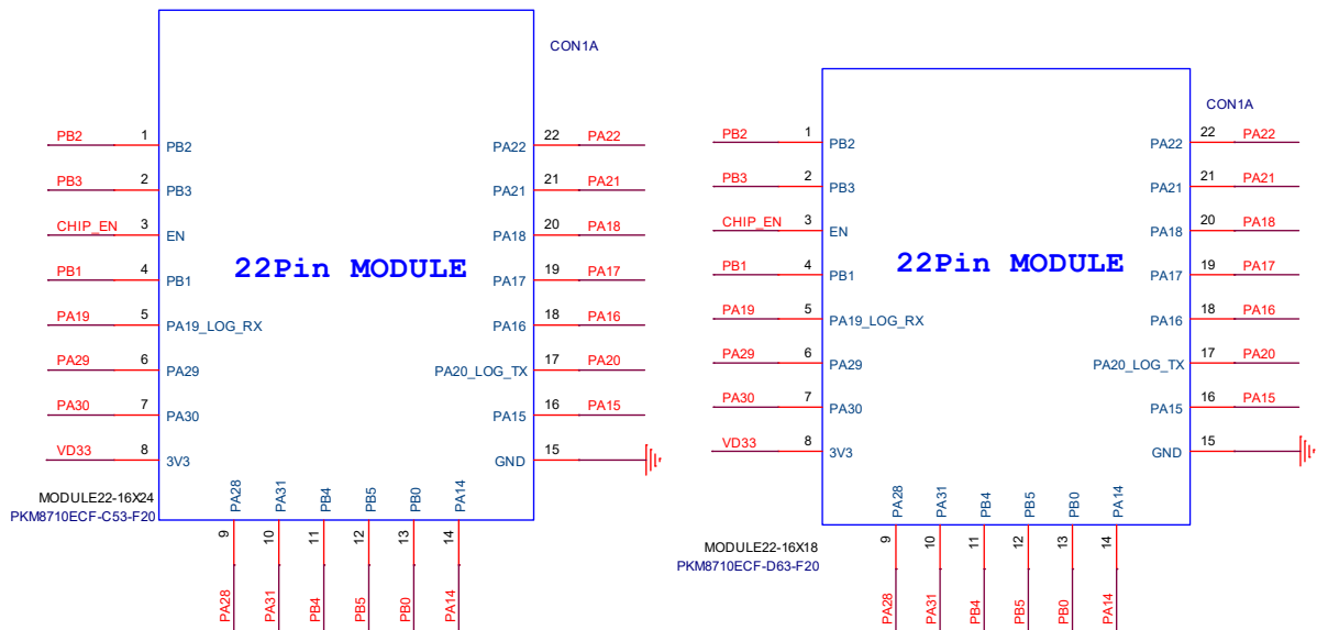
Figure 5. Module Reference schematics
