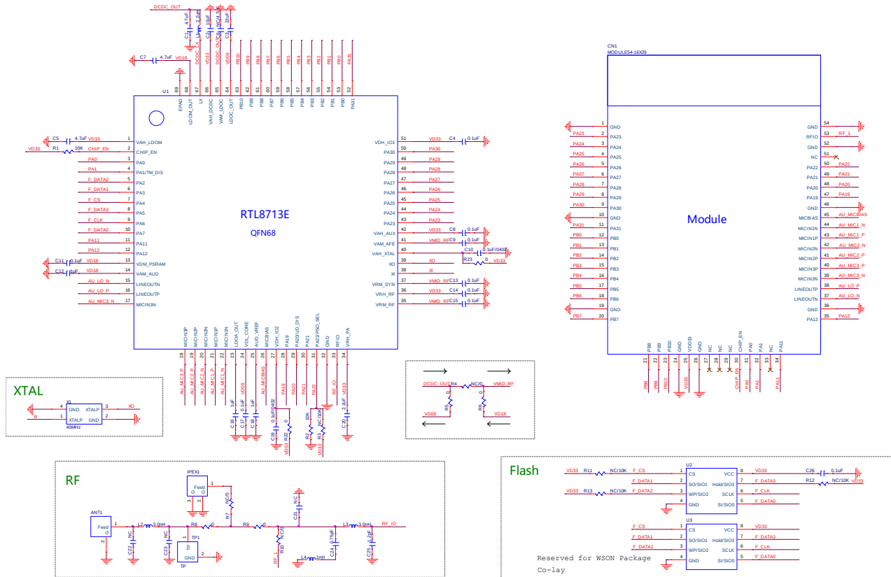
Figure 3. Module Internal Schematics
