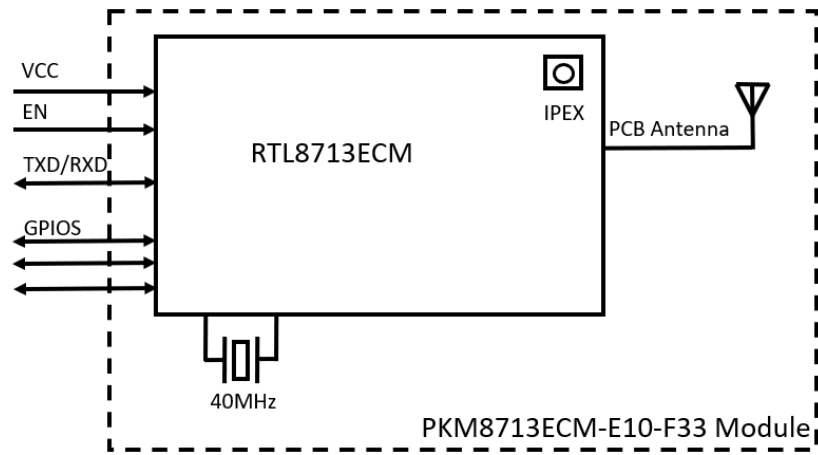
Figure 1. Block Diagram
