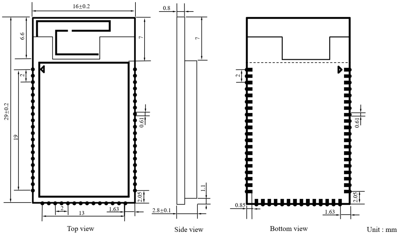
Figure 4. Module Physical Dimensions
