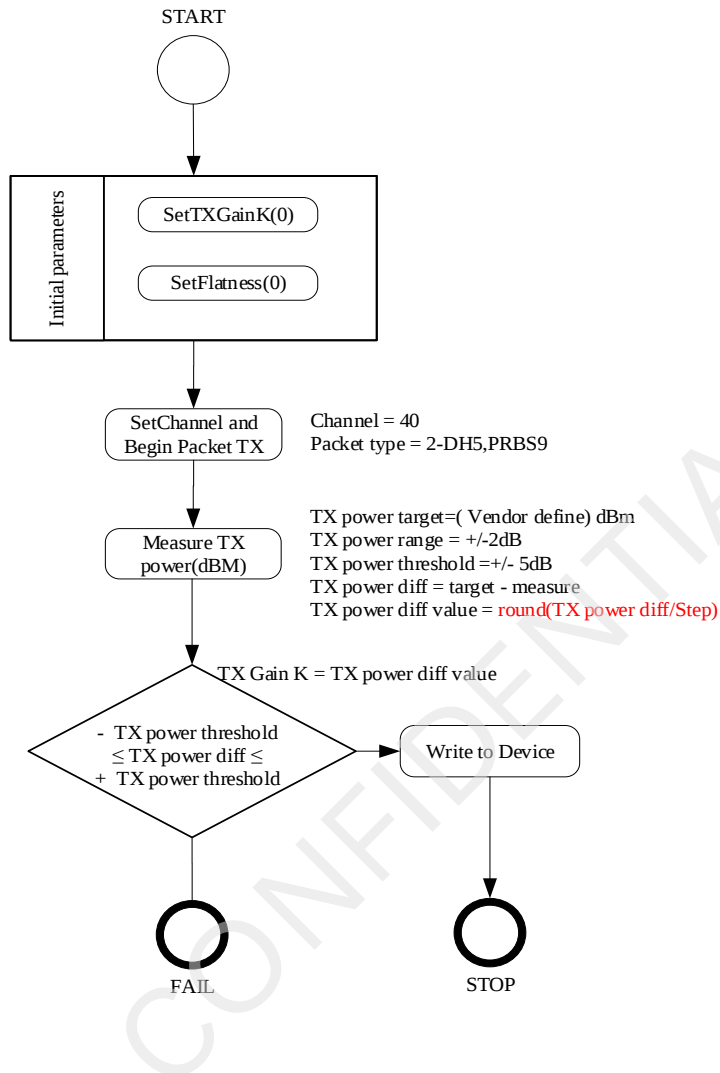
Figure 17: Calibration to Target Power
