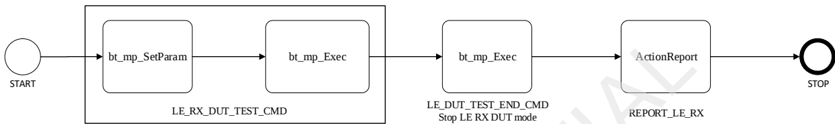
Figure 37: Start LE RX DUT test flow
