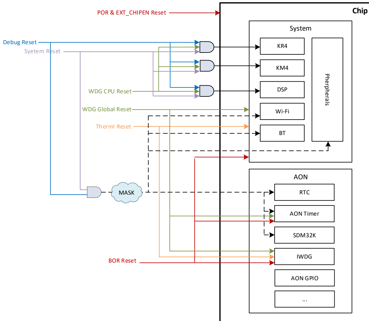
Figure 3-5 Reset diagram
