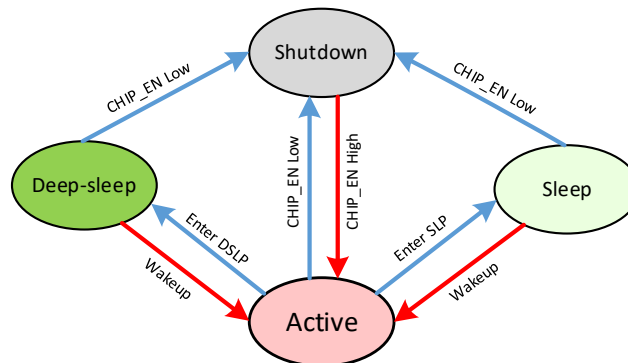
Figure 3-4 Switch among different power modes
