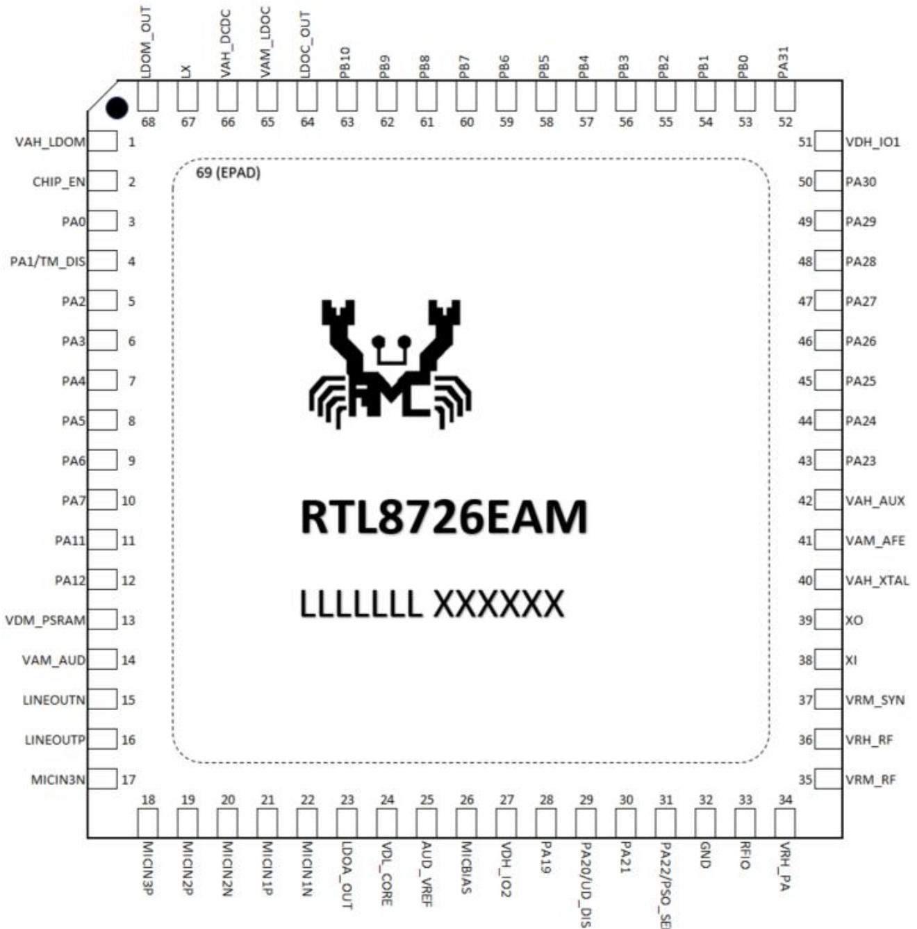
Figure 2-1 Pin assignments of RTL8726EAM series
