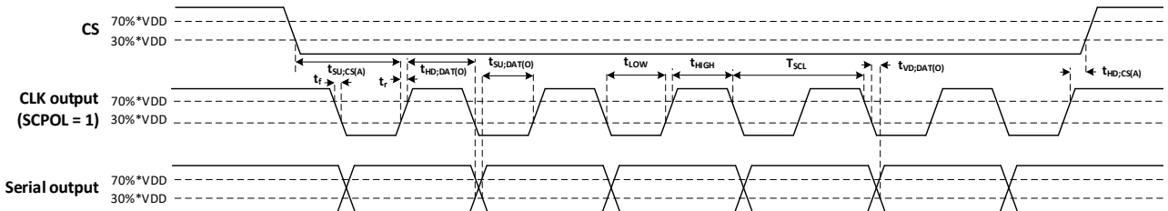
Figure 4-8 Output timing diagram (SCPH = 1)
