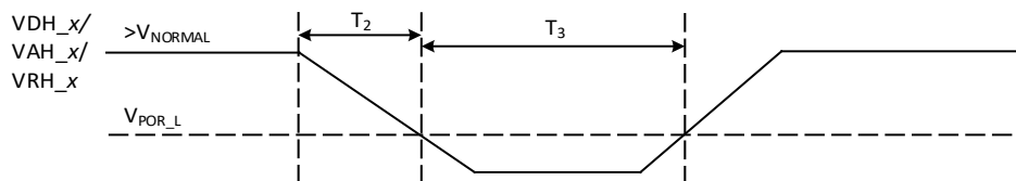
Figure 4-4 Power-off sequence
