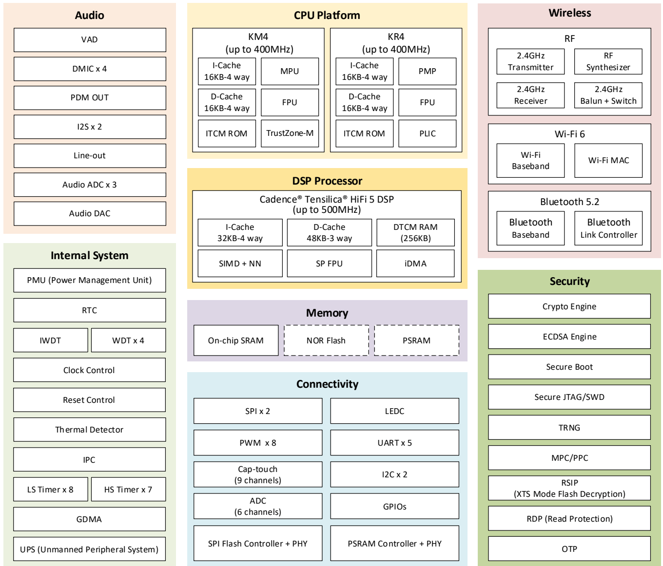
Figure 1-1 Block diagram
