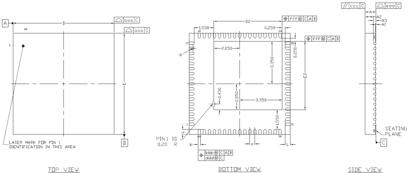
Figure 5-1 QFN68 package outline
