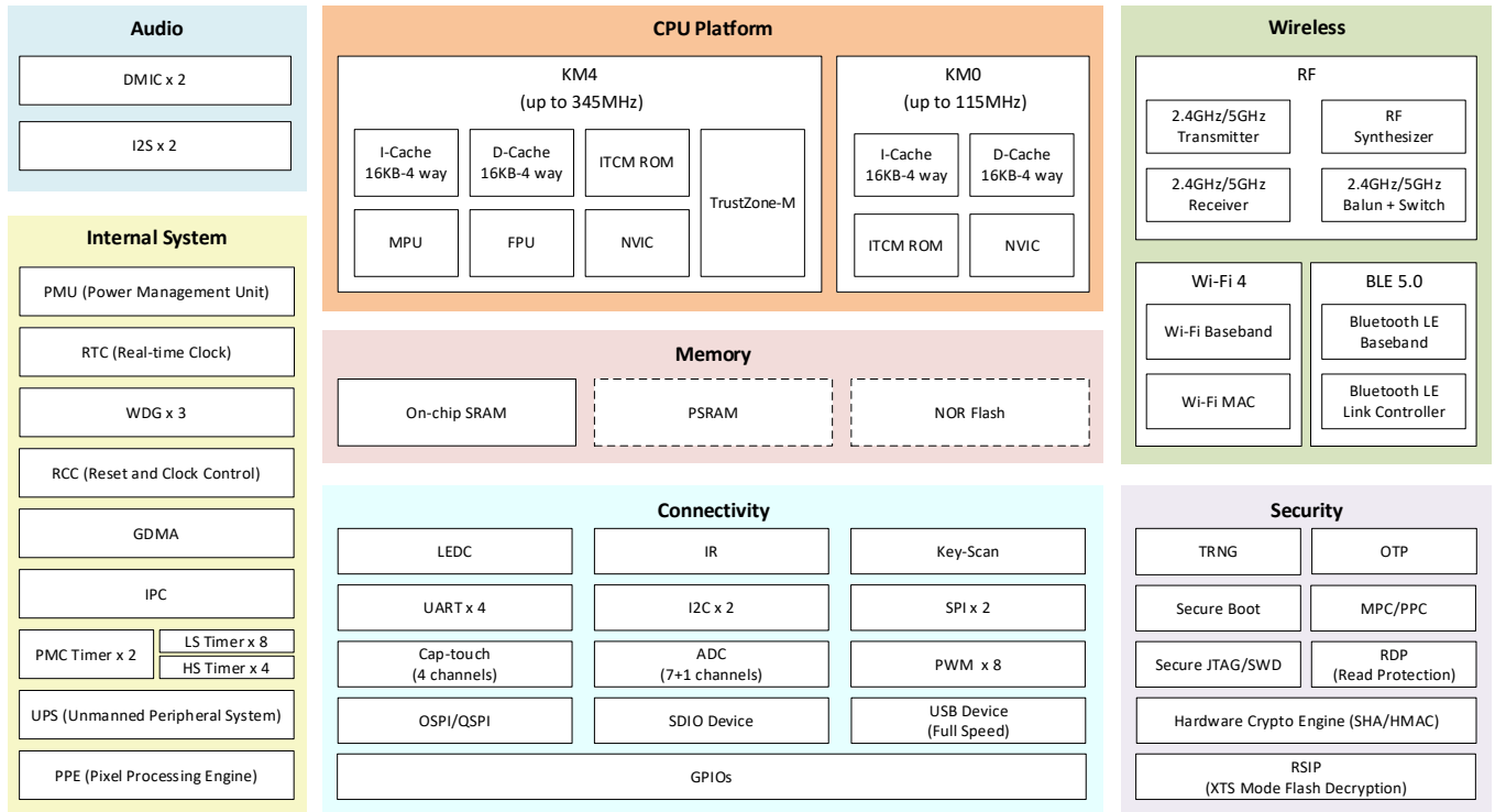
Figure 1-1 Block diagram
