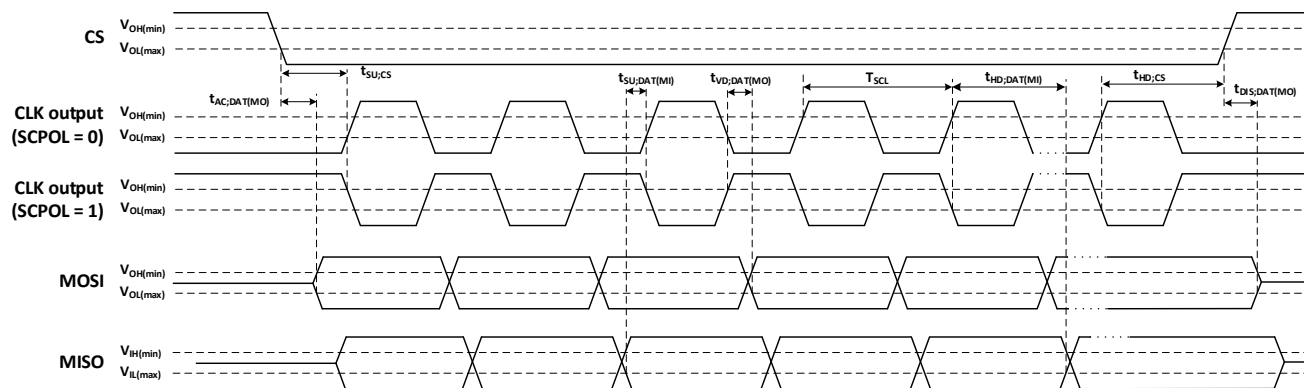
Figure 4-13 Timing diagram for master (SCPH = 0)
