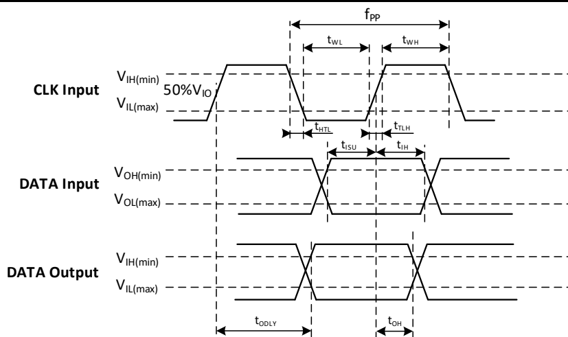
Figure 4-29 Timing parameters for SDIO device (high speed mode)
