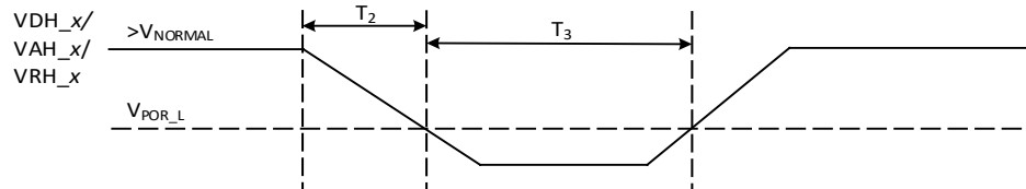
Figure 4-4 Power-off sequence
