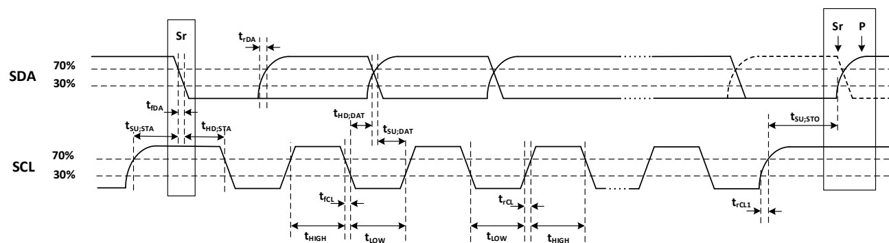
Figure 4-18 Timing diagram of I2C (HS mode)
