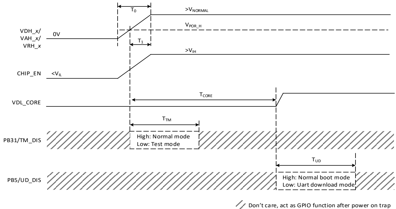
Figure 4-3 Power-on sequence
