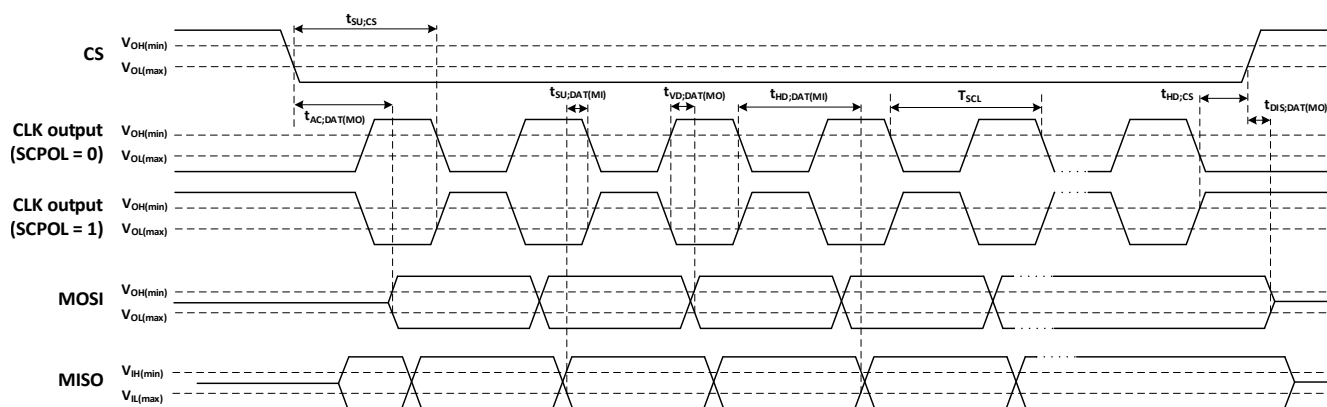
Figure 4-14 Timing diagram for master (SCPH = 1)
