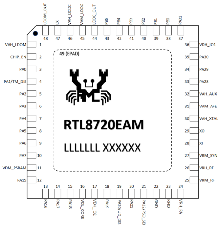
Figure 2-2 Pin assignments of RTL8720EAM series
