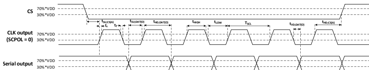
Figure 4-6 Output timing diagram (SCPH = 0)
