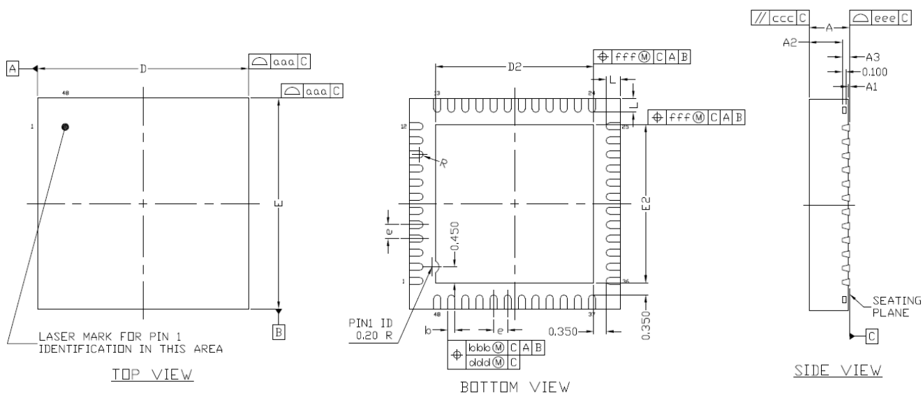
Figure 5-1 QFN48 package outline
