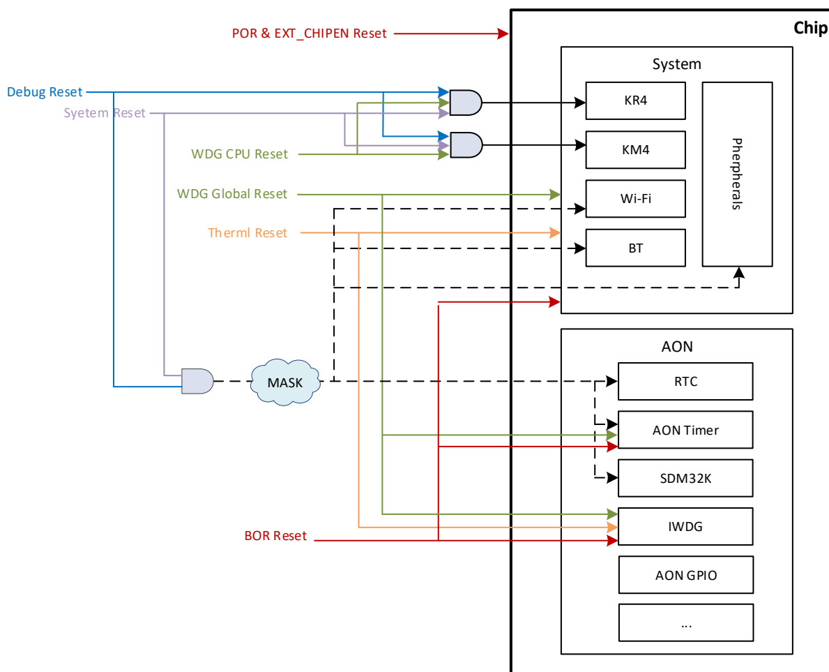
Figure 3-5 Reset diagram
