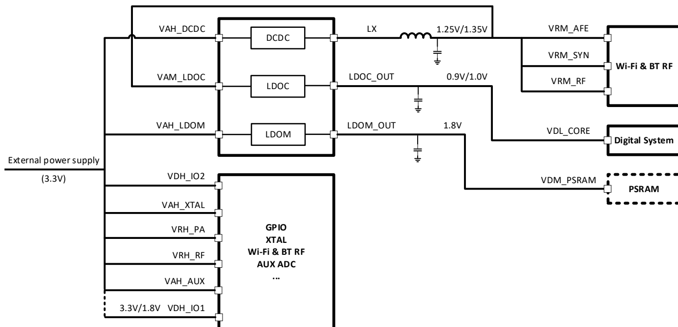
Figure 3-2 Power structure (power supply option 2)
