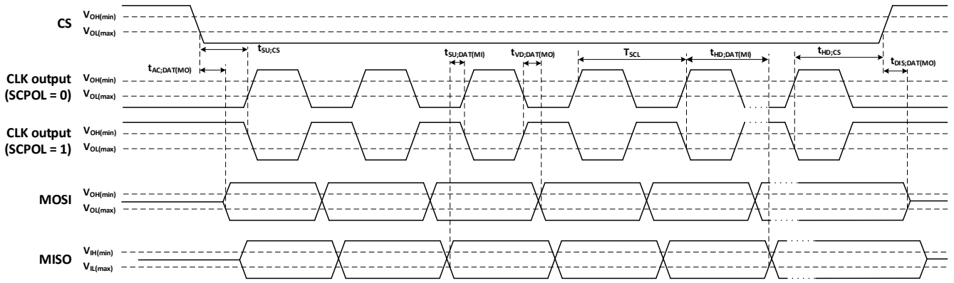
Figure 4-10 Timing diagram for master (SCPH = 0)
