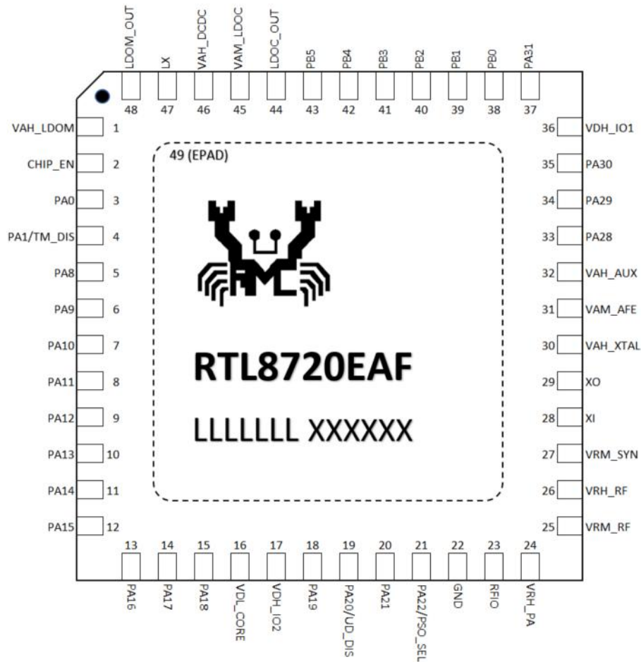
Figure 2-1 Pin assignments of RTL8720EAF series
