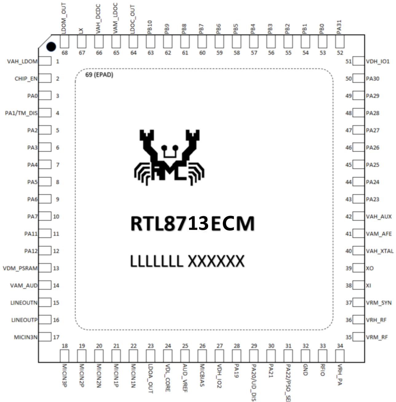
Figure 2-1 Pin assignments of RTL8713ECM series
